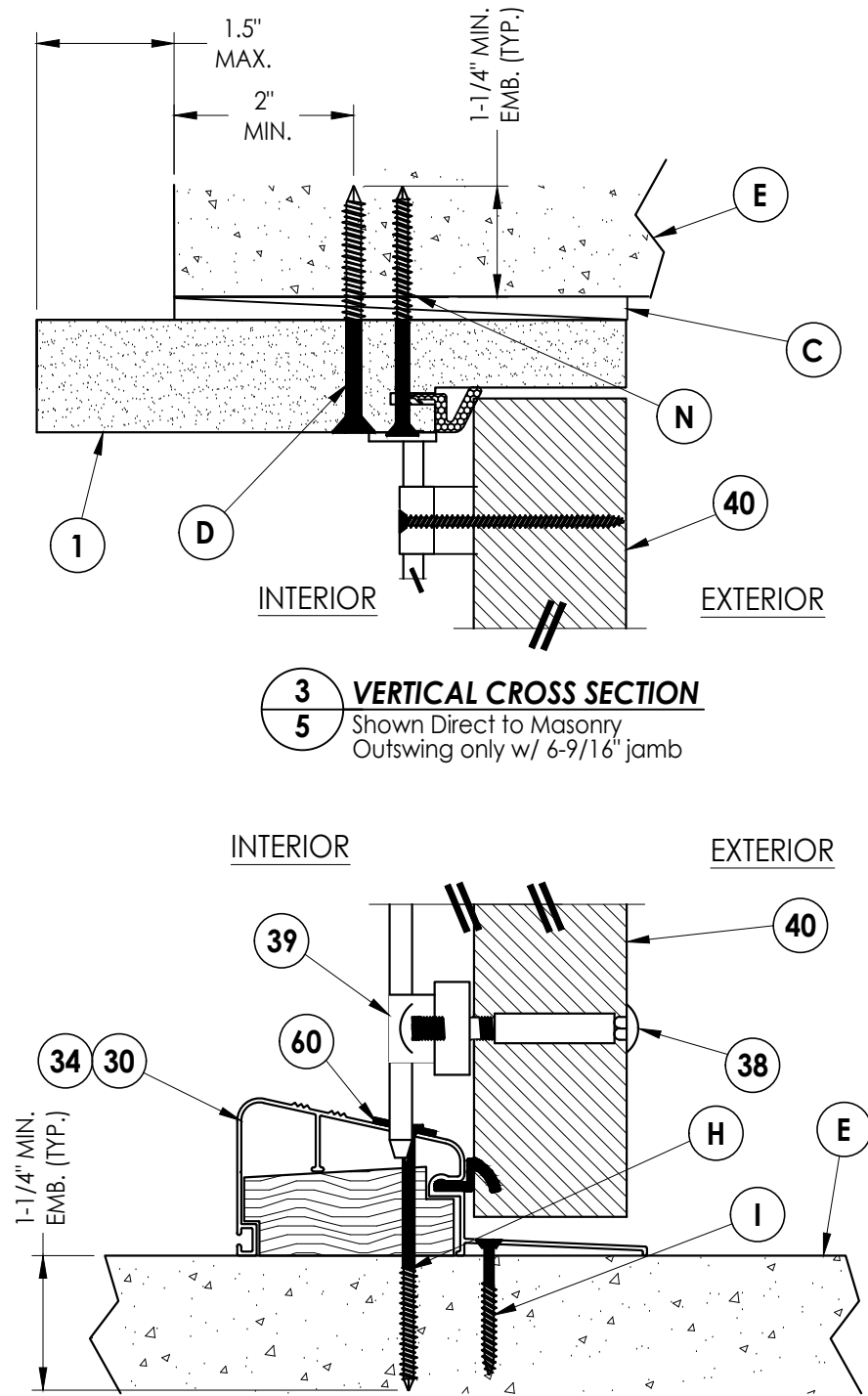
4 5 VERTICAL CROSS SECTION Shown Direct to Masonry
