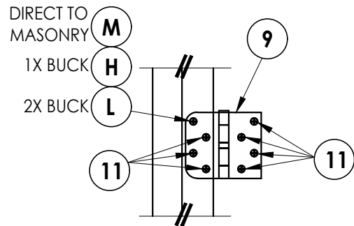
HINGE DETAIL
