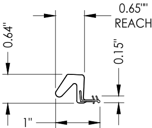
7 WEATHERSTRIP Endura Force 5
